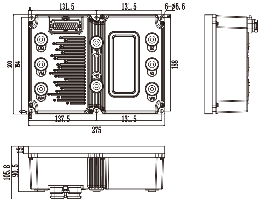
LC080350-350-R*N
