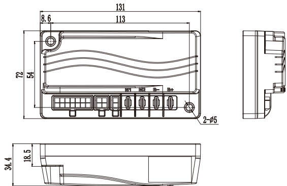
LC024025-BD
